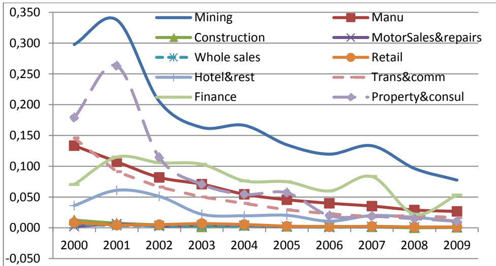
Figure 2: Industry Average PCM (2000–2009)
