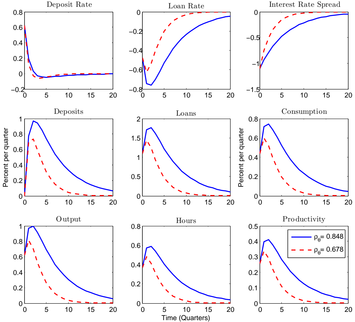
Figure 4: Impulse responses of one s.e positive credit shock ( \rho_\theta = 0.848 and 0.678 , \mu_\theta = 1 )
