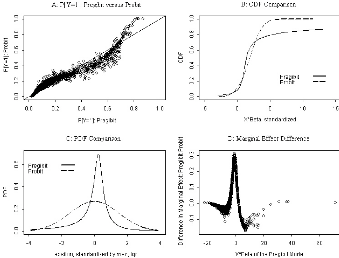
Figure 9: Differences between pregitbit and probit: denial of mortgage applications in the US
