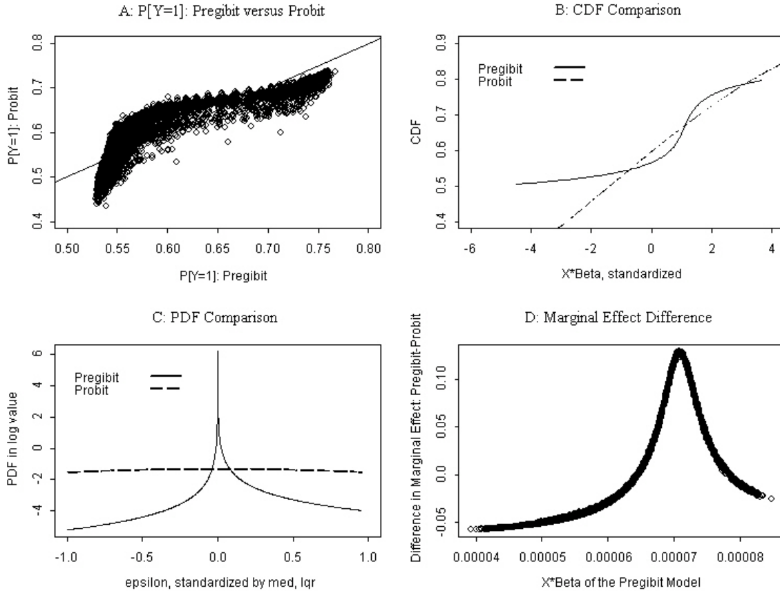
Figure 10: between pregibit and probit: doctor's visits in Germany
