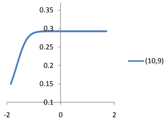
Figure B.4: GTL densities for (\alpha, \delta) = (10, 9)
