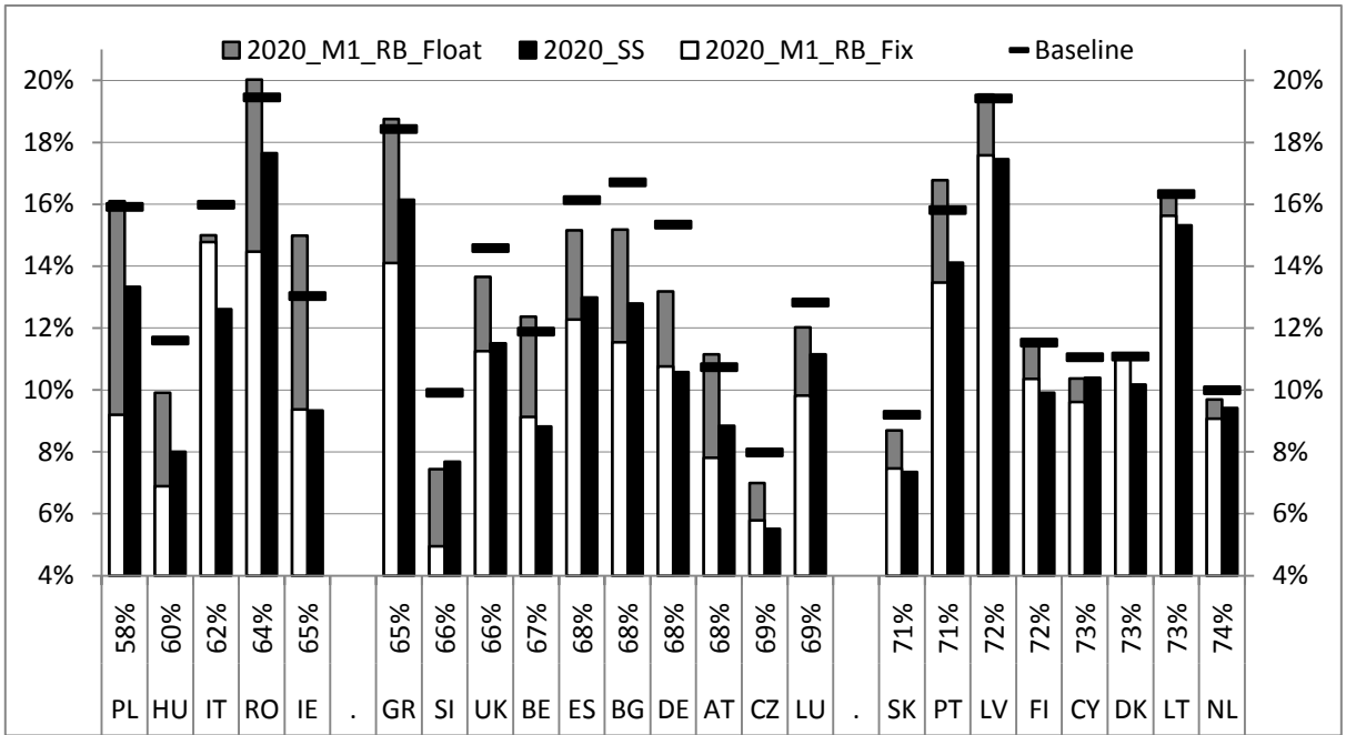
Figure 1. Poverty rates before and after increase of employment to 75% using shift-share and regression-based approach (fixed and floating poverty line), active age population
