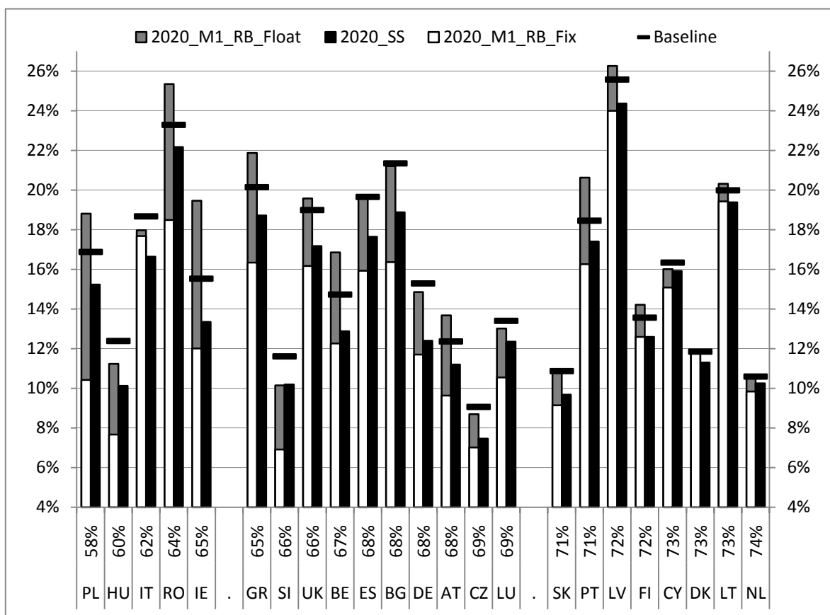
Figure A.1. Poverty rates before and after increase of employment to 75% using shift-share and RB approach (fixed and floating poverty line), entire population, poverty line at 60% of median equivalent income, 2008
