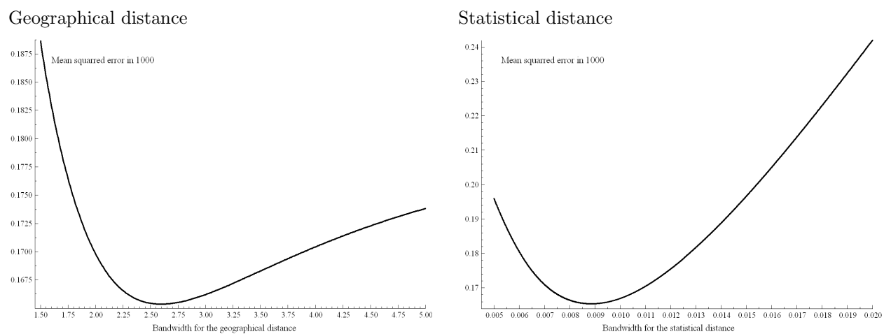
Figure 1. Convexity of cross validation function
