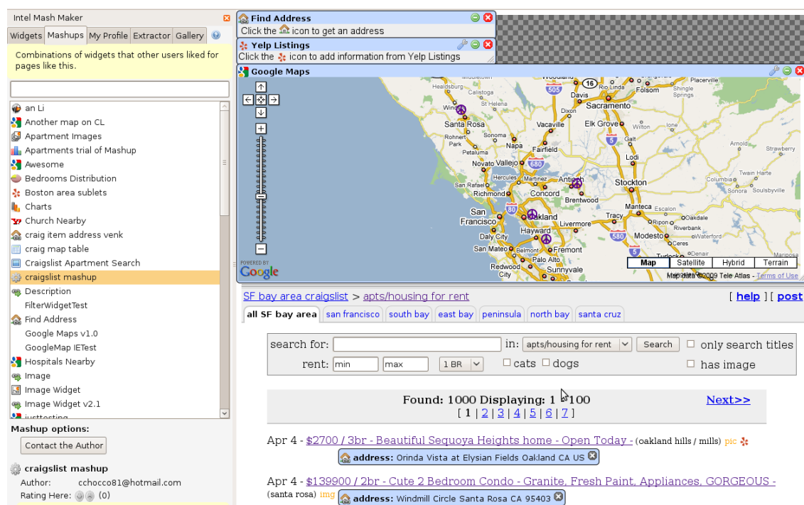
Figure 8: Mash Maker mashup showing craigslist entries on a map.
