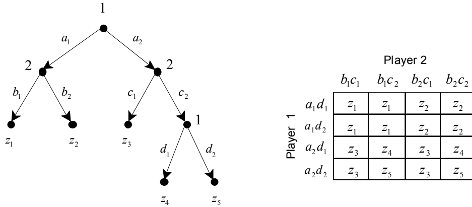
(a) A perfect-information game (b) The corresponding strategic form
