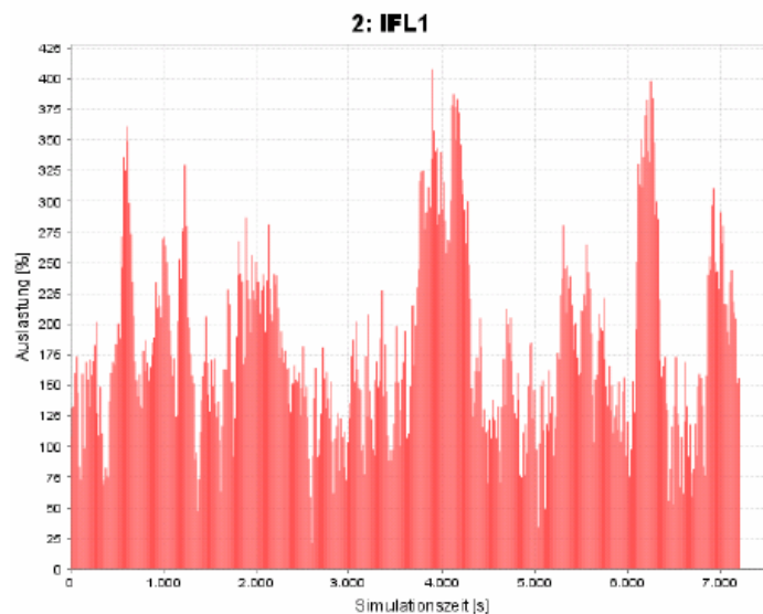
Figure 10: Time dependent utilization for an IFL-processor
