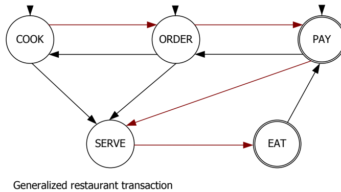
Figure 15: Generalized state chart and included “specialized” process – adapted from (Wyner and Lee 1994)
