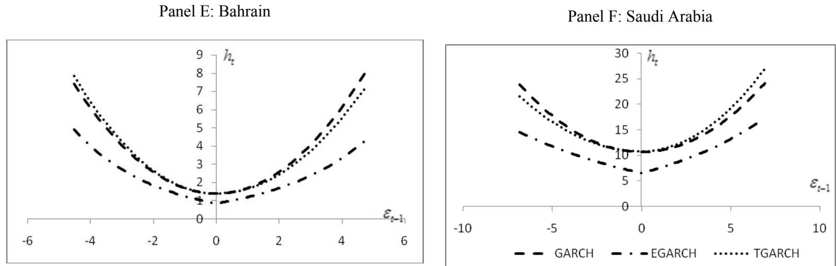
Figure 2: News impact curve all GCC markets of symmetric and asymmetric models
