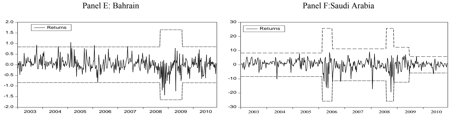
Figure 1: Weekly GCC stock price returns
