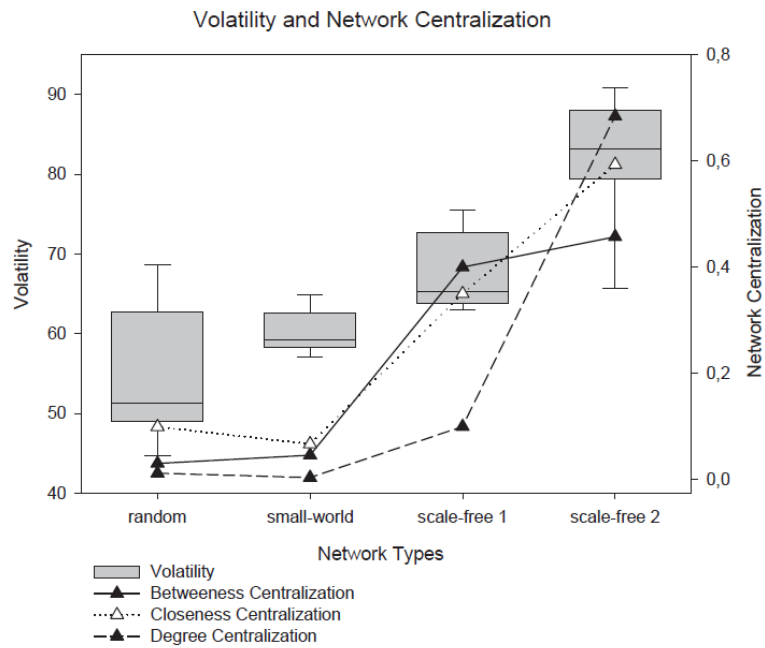
Figure 5: Results for the volatility in relation to network centralization
