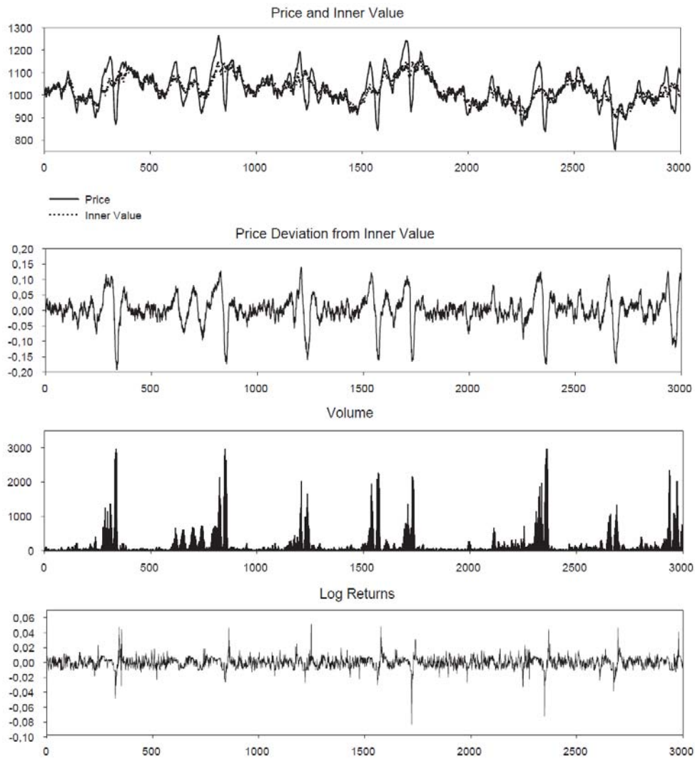
Figure 2: Simulation results using the small-world communication network.
