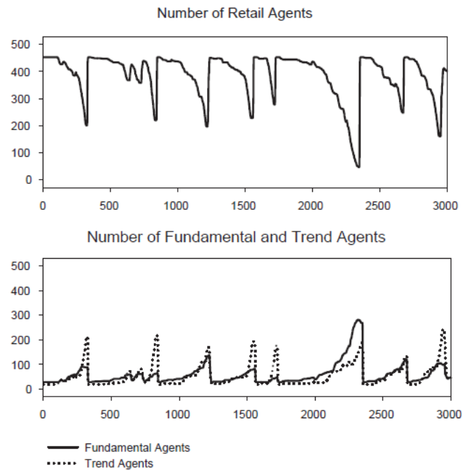
Figure 4: Results for the group sizes of retail, trend and fundamental agents using the small-world network
