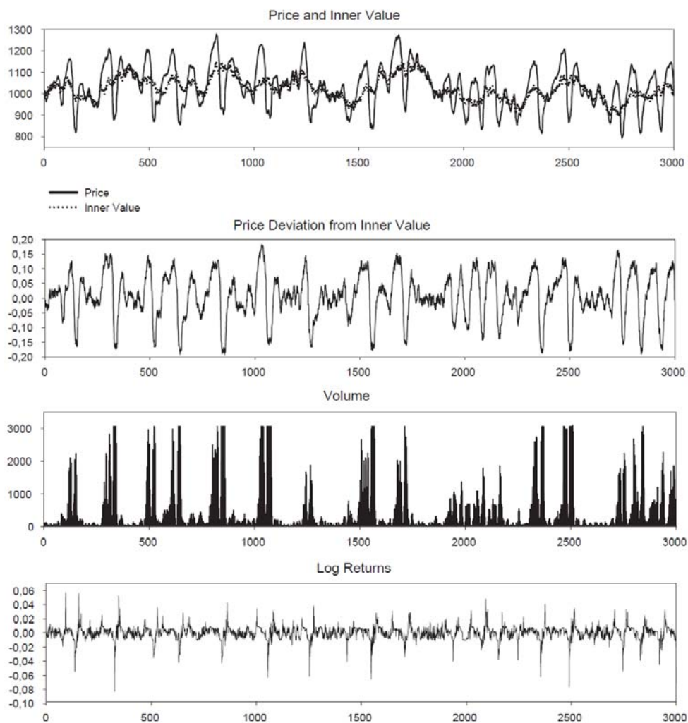
Figure 3: Simulation results using the scale-free 2 network
