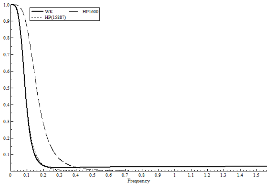
Figure 5: Gain functions of WK, HP(1600) and HP(15887) filters (RW(2); AR(2), \varphi_1 = 1.765 , \varphi_2 = -0.81 )
