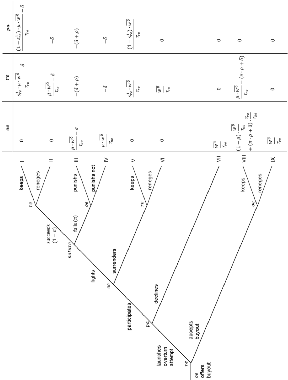
Figure 4: Revolution Game
