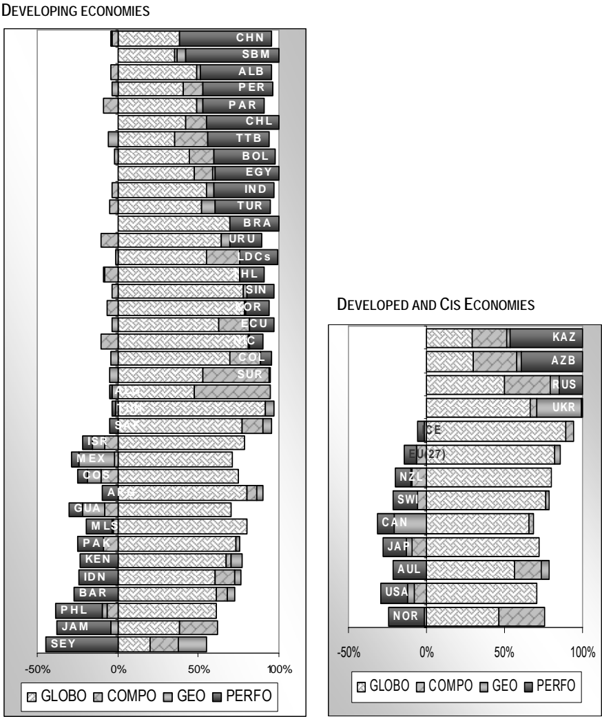
Chart 1. Shift-Share Analysis of Developing, Developed and CIS economies, 2002-2007
