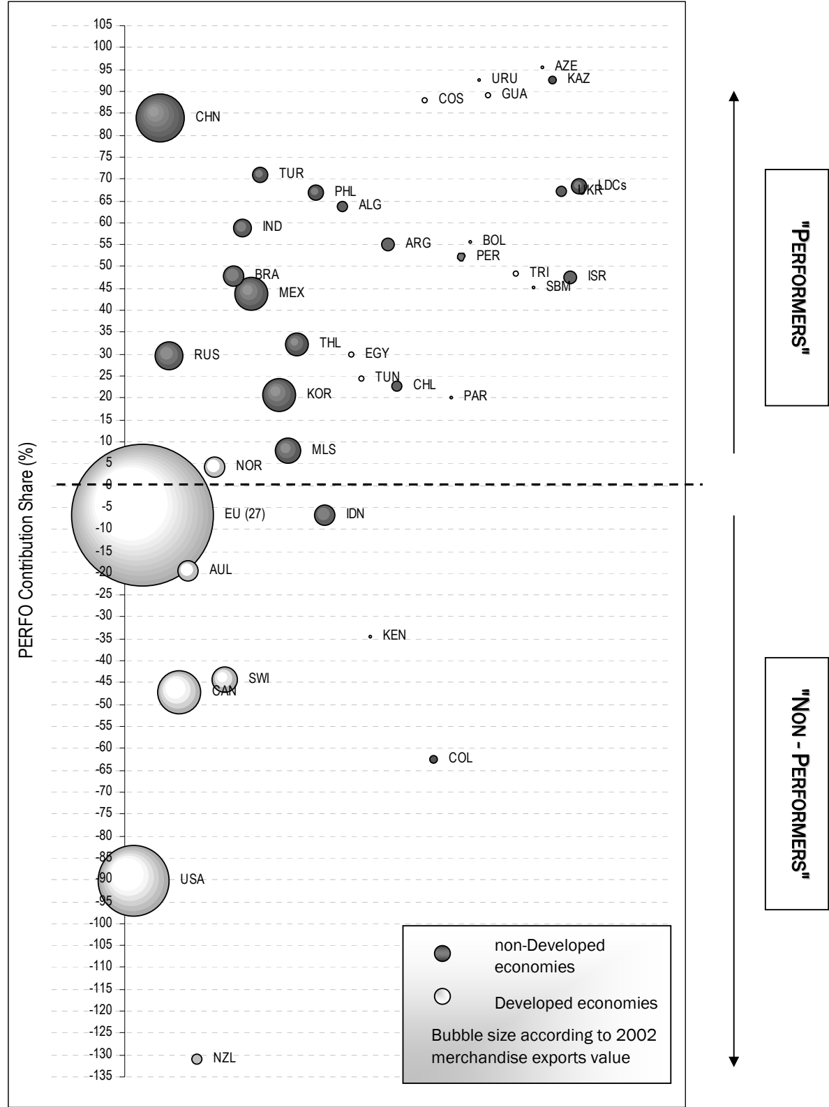
Chart 2. Shift-Share Analysis of selected economies, 1996-2002 (Percentage)
