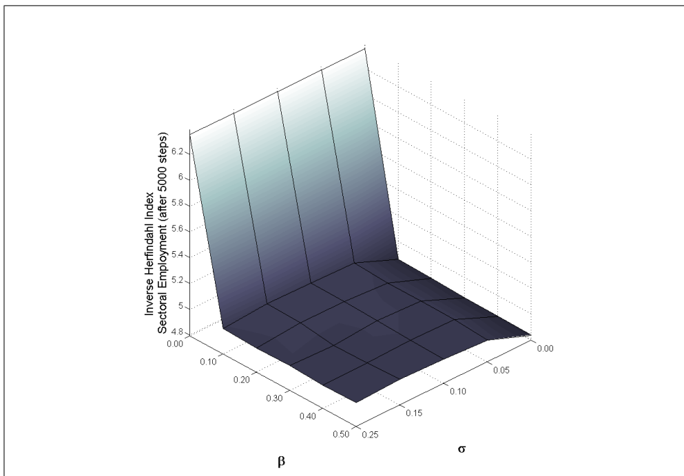
Figure 19: Employment concentration \mathcal{H}_{L,t} ; \sigma vs. \beta ( t=5000 ): This figure includes the case in which \delta = 0.00 . Structural change does not occur and the concentration in employment remains unchanged.
