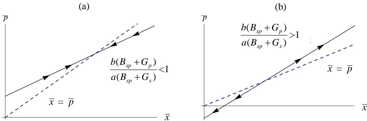
Figure 1 The phase plots of the model's evolutionary learning trajectories for (a) a > b and (b) a < b ( B_{xp}=3, G_x=1, G_p=1 ).
