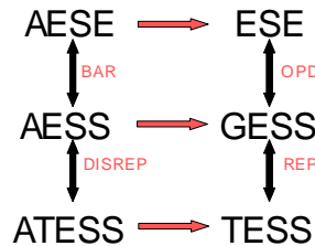
Figure 3: Overview of equivalences shown, arrows denote inclusions: red for general, black for special dynamics. BAR denotes the barycentric projection dynamics of Prop. 5, DISREP denotes disturbed replicator dynamics, containing at least the dynamics in Prop. 7 & 8.
