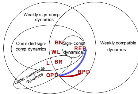
Figure 2: Relations between dynamics. The red line depicts barycentric ray-projection dynamics; the blue one q -deformed replicator dynamics, q \in [0, 1] .
