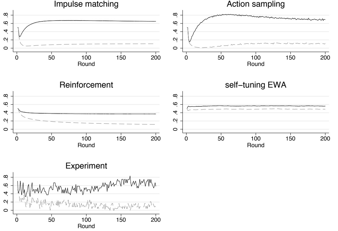
Figure 5: Mean probabilities for left and right in the simulations runs and the experiment for game 7 . Mean probability for left is given in black and the mean probability for up is given in gray.
