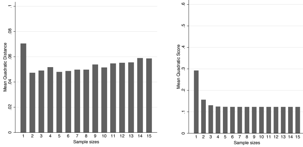
Figure A.15: Figure gives the mean quadratic distance (left) and the mean quadratic score (right) of payoff-sampling for different sample sizes
