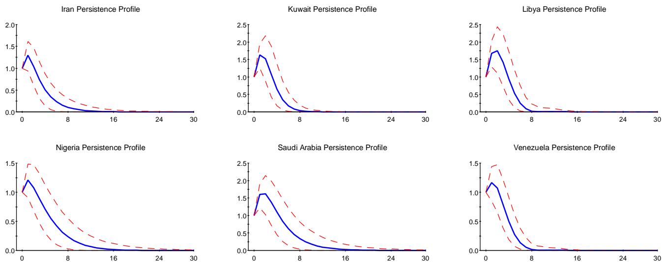
Figure 2: Persistence Profiles of the Effect of a System-wide Shock to the Cointegrating Relation (with 95 percent bootstrapped confidence bounds)
