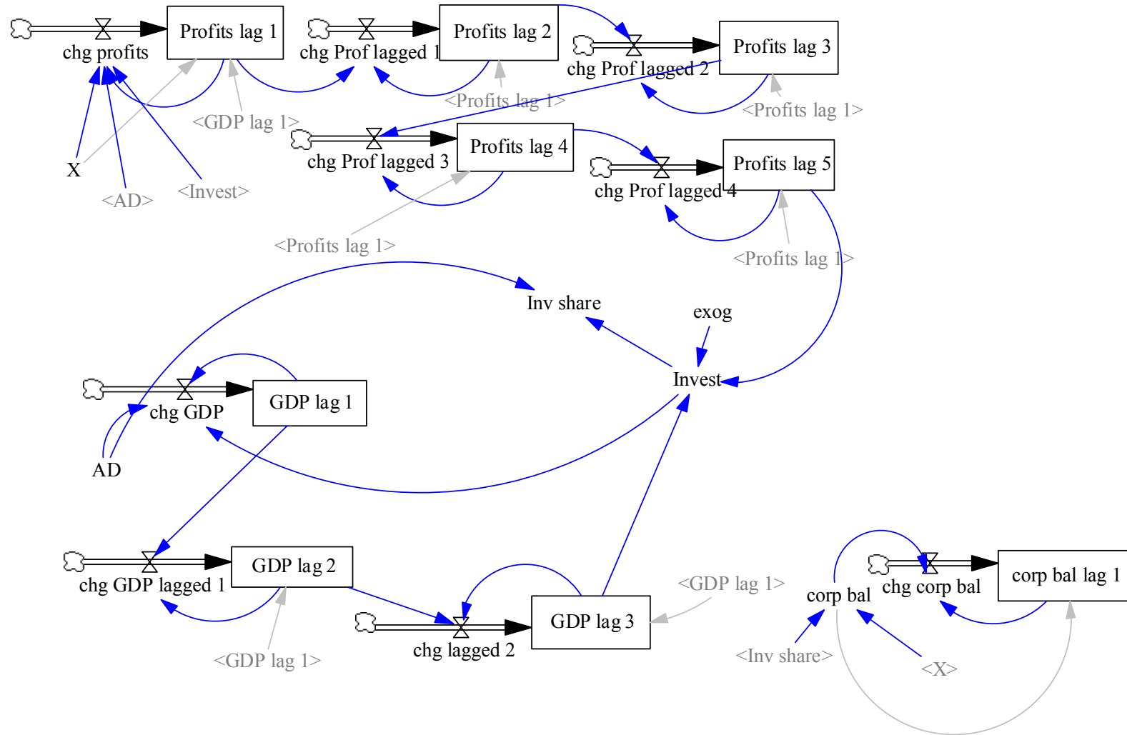
Figure D1: Simulation Model with Exogenous Profits Share
