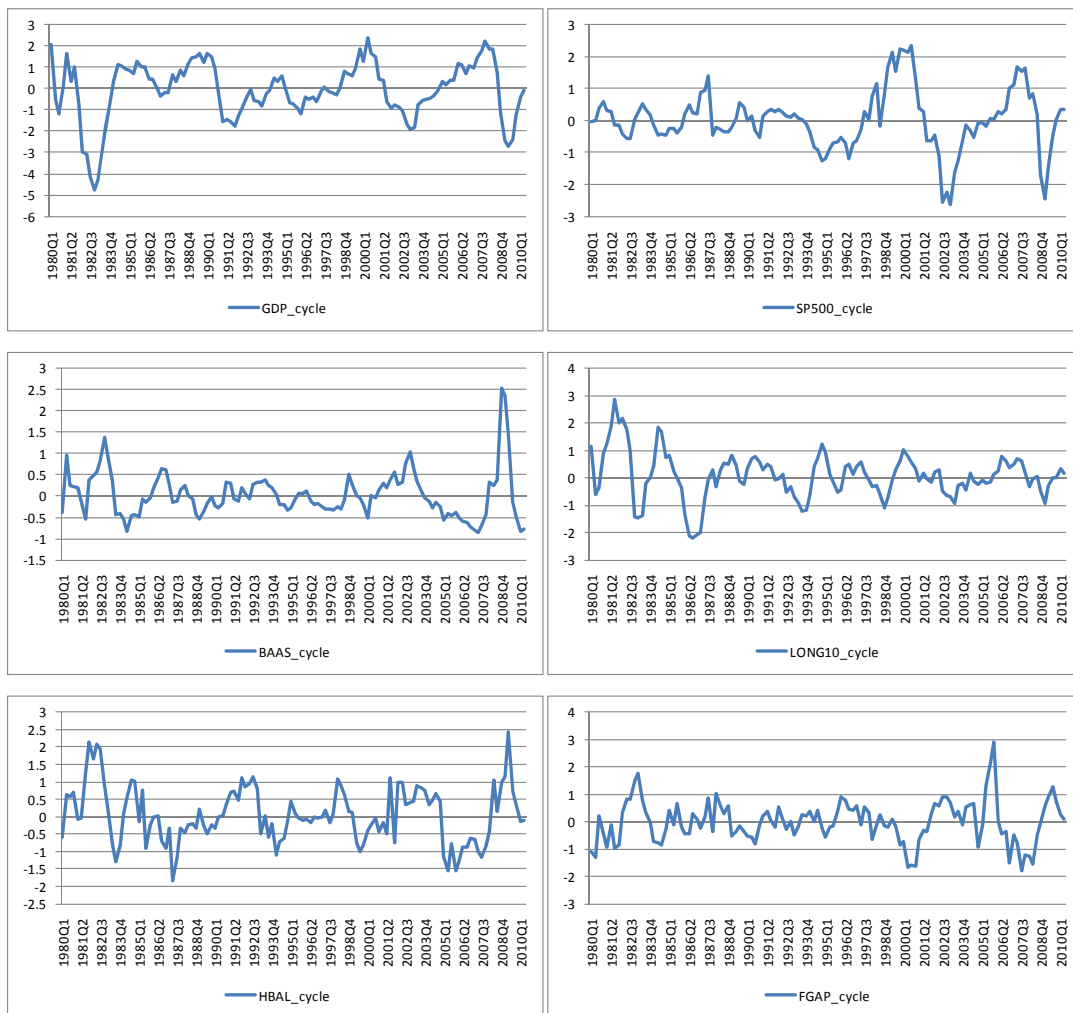
Figure 3: Time Series Used in VAR Estimation, 1980q1–2010q2
