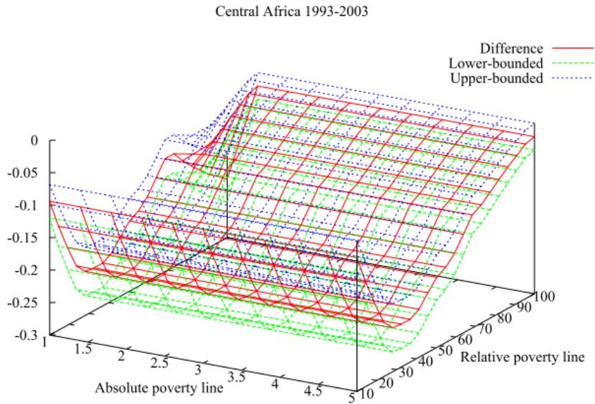
Figure A2: Bidimensional growth dominance
