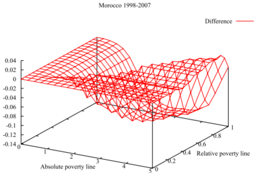
Figure A14: Bidimensional growth dominance curves
