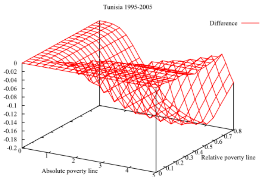
Figure A18: Bidimensional growth dominance curves
