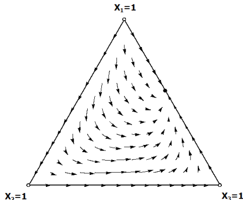
Figure 4 Travelers' Dilemma played by partially observed level- k types. Parameters R = 3/2 , P = 1/3 , and n = 6 . Type space K = \{1, 2, 3\} . The state with x = (4/7, 0, 3/7) (black dot) is asymptotically stable and has the whole interior as its basin of attraction.
