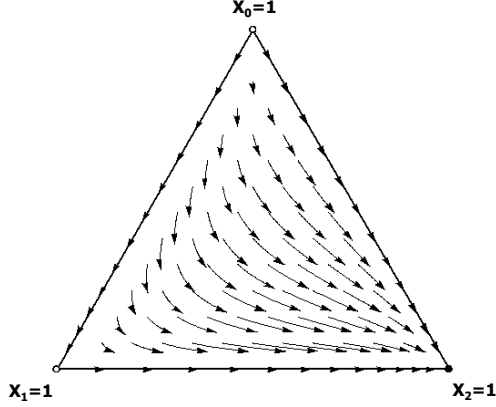
Figure 1 Travelers' Dilemma played by level- k types. Parameters R = 3/2 , P = 1/3 , and n = 6 . Type space K = \{0, 1, 2\} . The state with x_2 = 1 (black dot) is asymptotically stable and has the whole interior as its basin of attraction.
