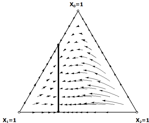
Figure 2 Hawk Dove played by level- k types. Parameter b = 2 , and type space K = \{0, 1, 2\} . The set X^* = X^{ESS}(K) (thick line) is asymptotically stable and has the whole interior as its basin of attraction.
