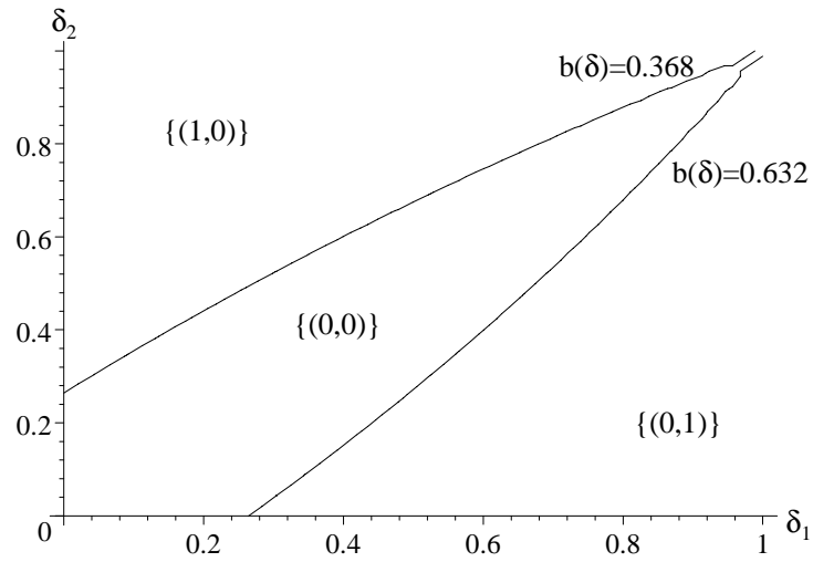
The discrete case when p = 3/4 .
