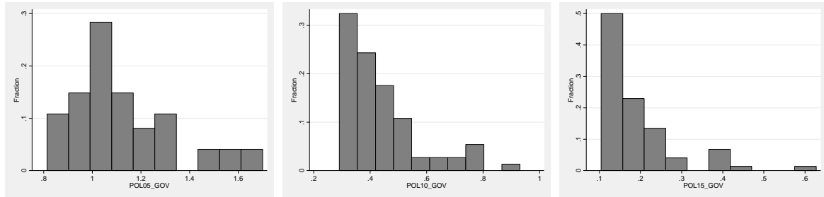
Figure 3. Histogram of Esteban and Ray’s polarization measure for the government responsibility question (GOV) for \alpha = 0.5 (left), \alpha = 1.0 (center) and \alpha = 1.5 (right).
