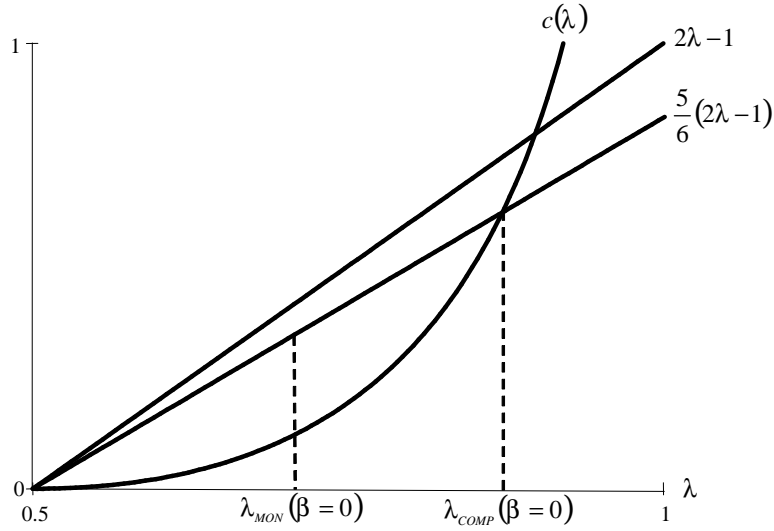
Figure 1: The cost function and IT 's revenue when \beta = 0 and \beta = 1 .
