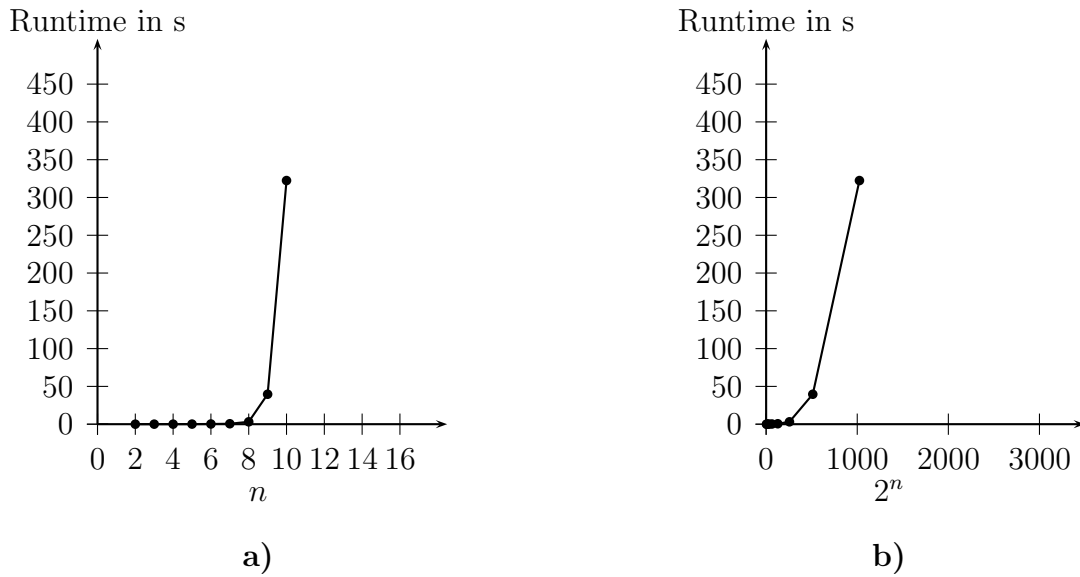
Figure 5: Runtime of our algorithm to compute all minimal sCURB sets in random games with n players and two strategies per player a) with respect to n , b) with respect to 2^n
