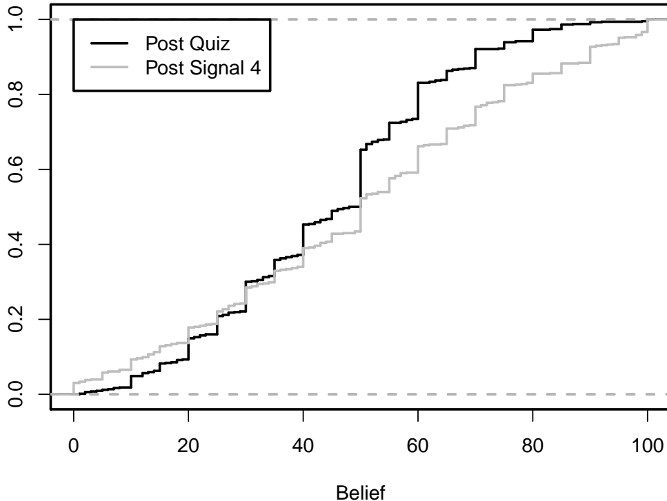
Figure 5: Belief Distributions
