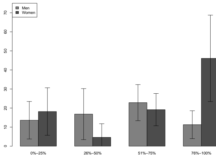
Figure 8: Information Values by Beliefs and by Gender
