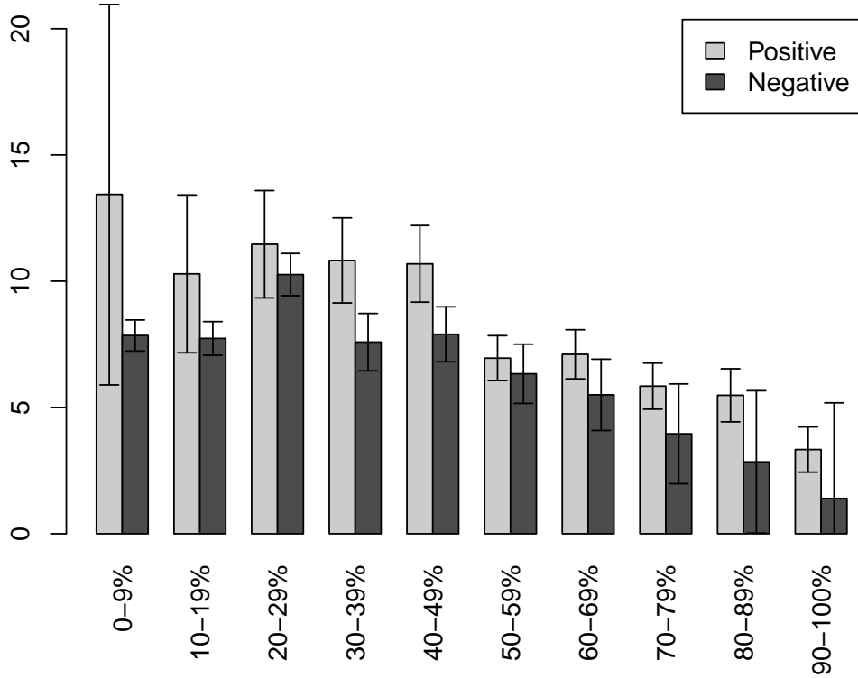
Figure 7: Asymmetry
