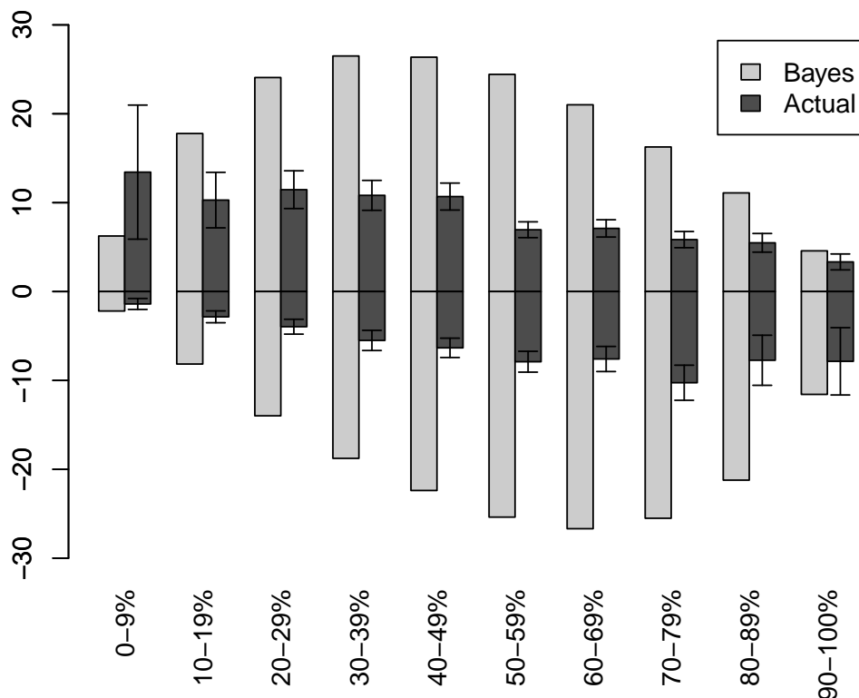
Figure 6: Conservatism
