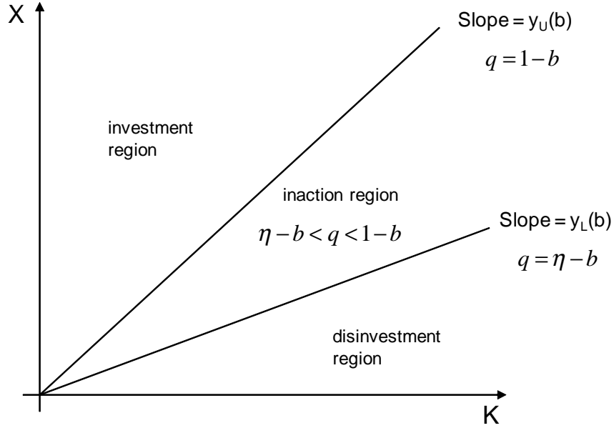
Figure 2: Projection of investment and inaction regions on the K - X plane. The line with slope y_U(b) gives the investment boundary, while the line with slope y_L(b) gives the disinvestment boundary. These two boundaries enclose the inaction region for investment. Source: Author's calculations.
