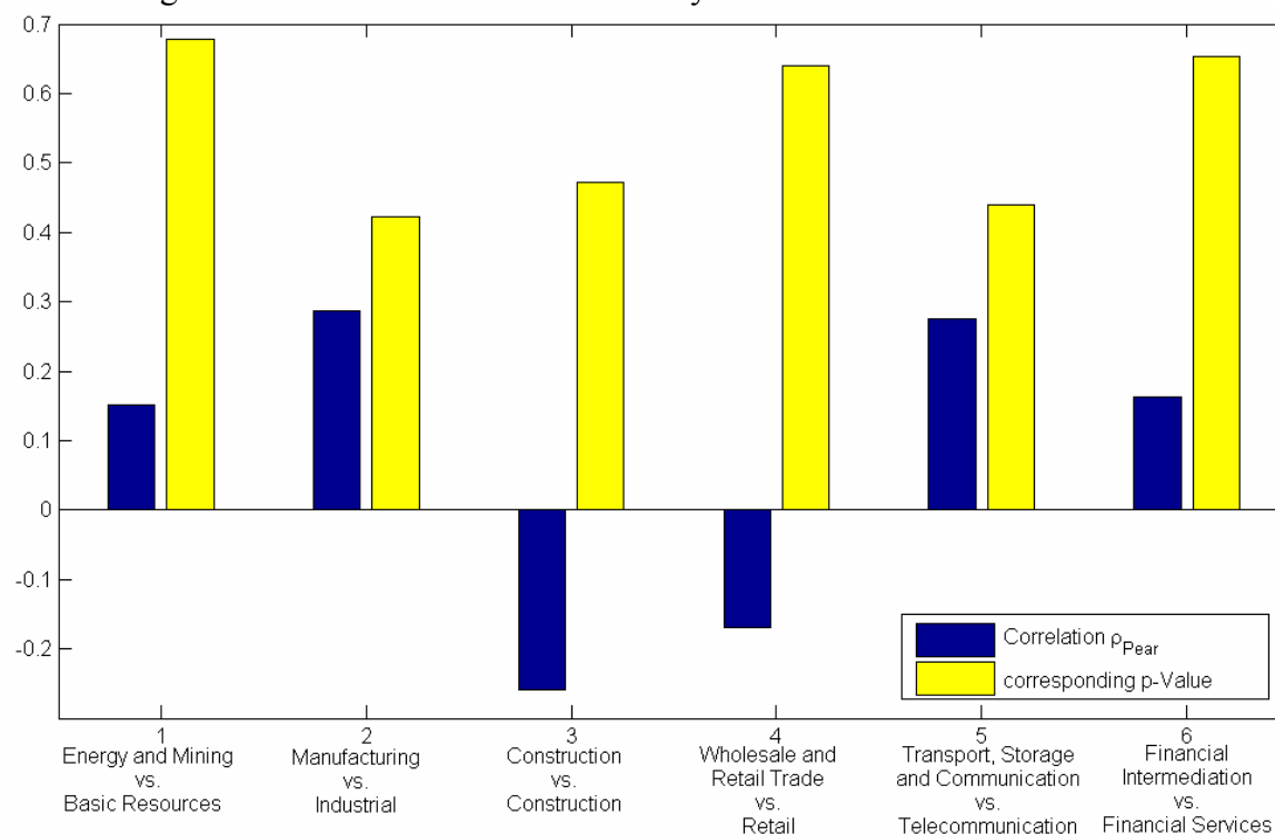
Figure 3 Correlations between Sector Systematic Factors and Prime Indexes
