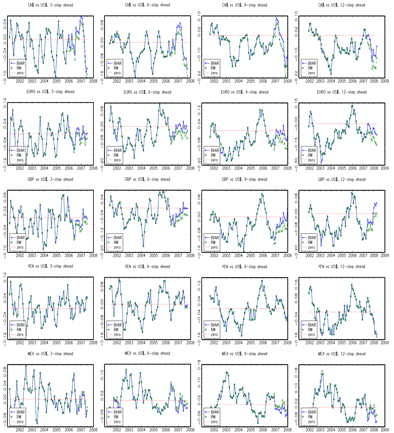
Figure 2: Forecasts Errors for different forecast horizons.
