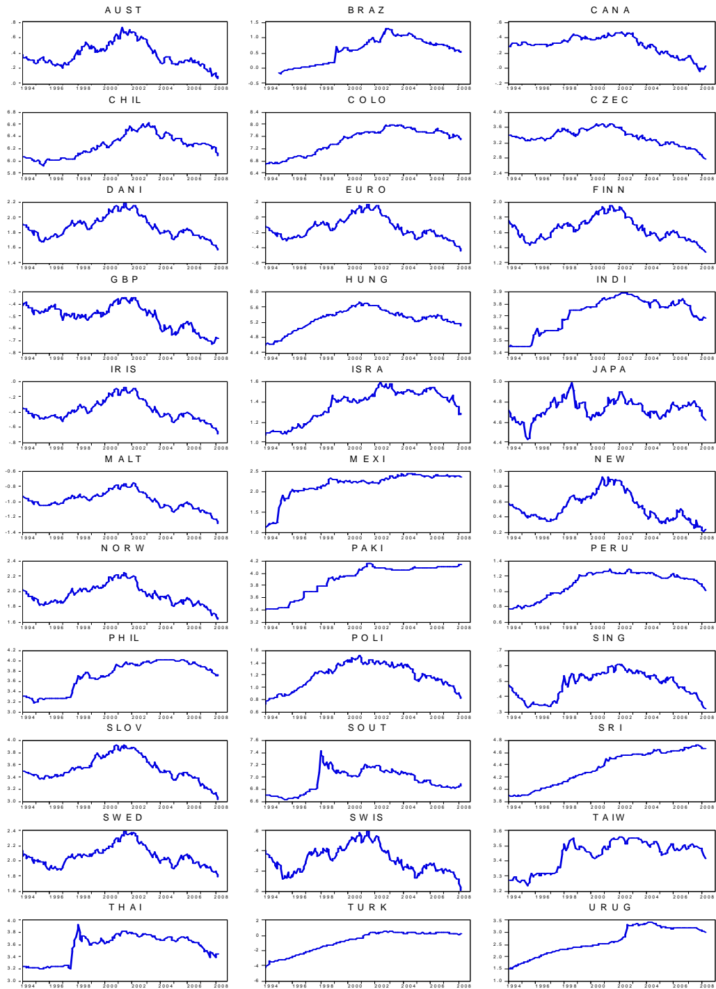
Figure 1: Monthly Exchange Rate Data (in natural logarithms).
