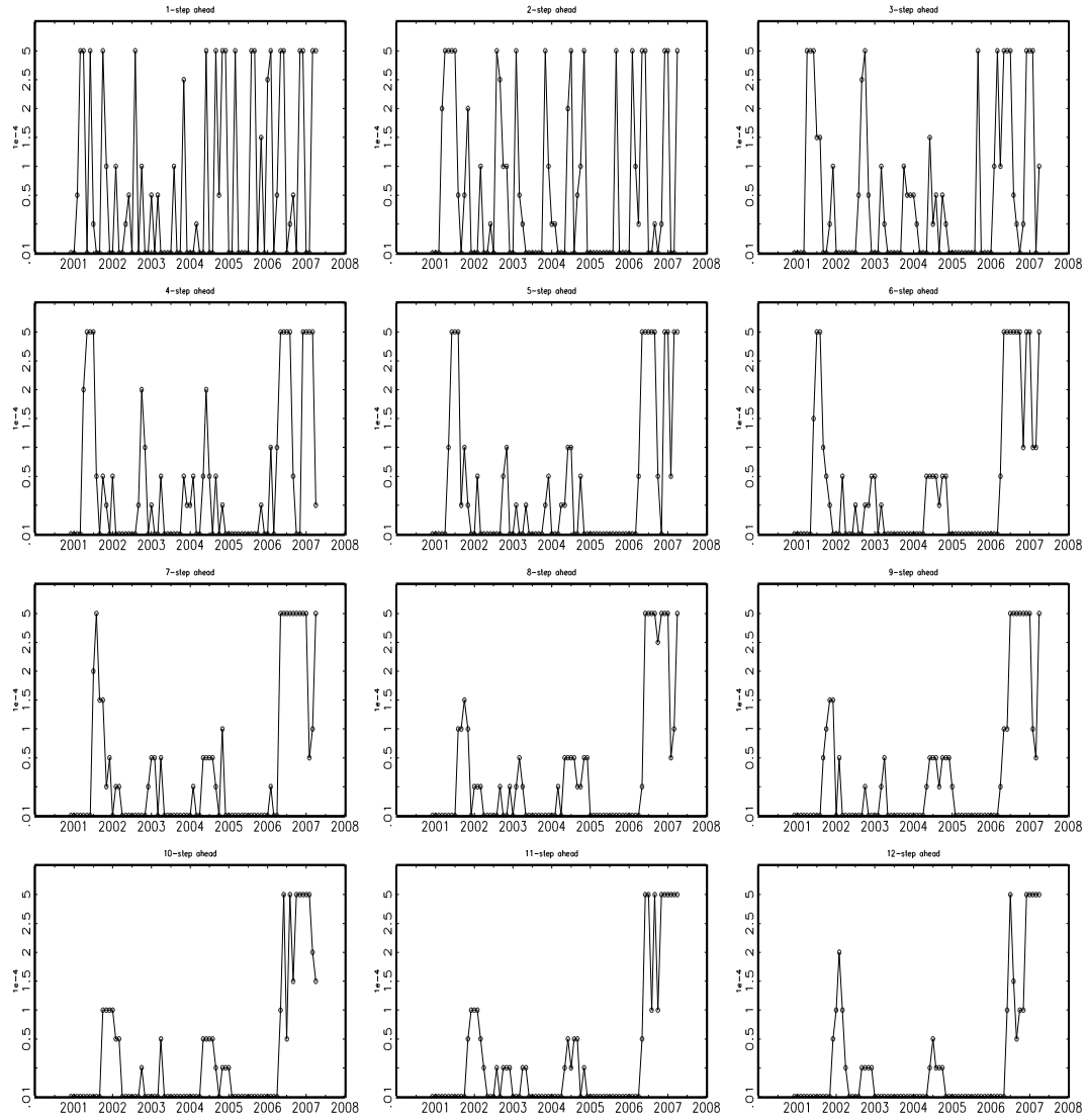
Figure 3: Selected value of the tightness parameter \theta , over time.
