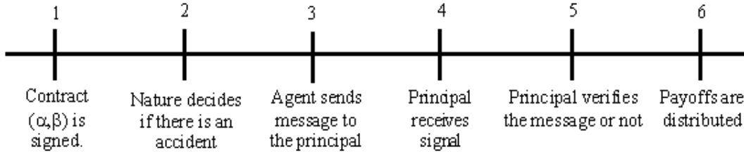
Figure 1: Sequence of play.
