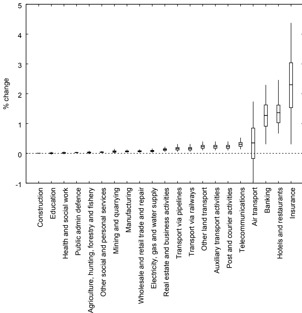
Figure 5: Means 50 and 95 Percent Confidence Intervals of the Sample Distributions of the Output Changes by Sector from Armenian-CISFTA—30,000 simulations.
