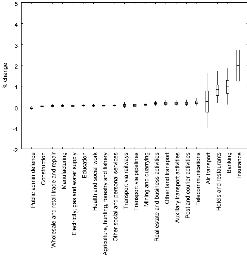
Figure 6: Means 50 and 95 Percent Confidence Intervals of the Sample Distributions of the Labor Payment Changes by Sector from Armenian-CIS FTA—30,000 simulations.
