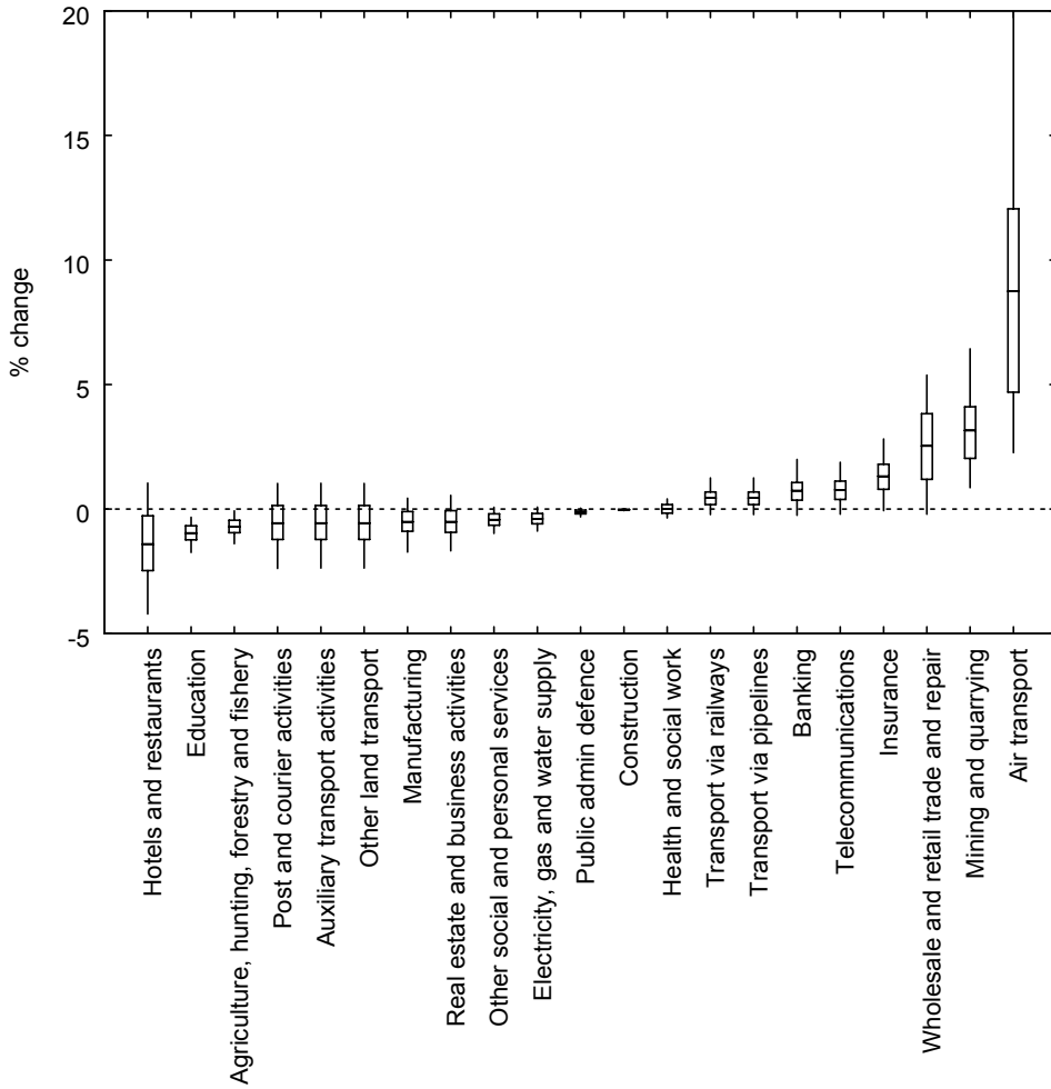
Figure 2: Means, 50 and 95 Percent Confidence Intervals of the Sample Distributions of the Output Changes by Sector from Armenian-EU DCFTA—30,000 simulations.
