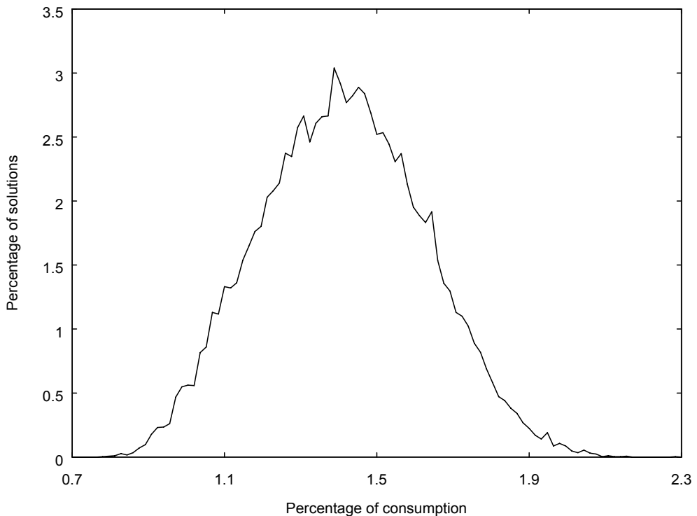
Figure 1: Sample Distribution of the Welfare Results of Armenian-EU DCFTA 30,000 simulations.
