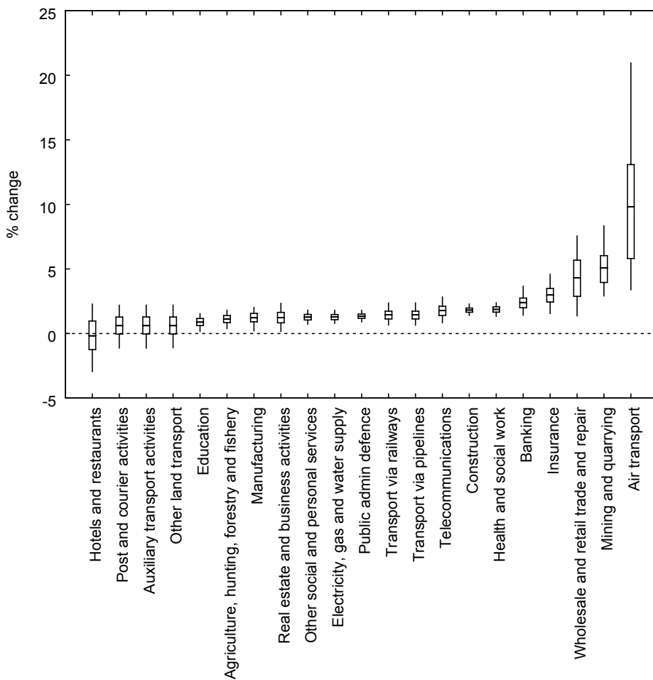
Figure 3: Means 50 and 95 Percent Confidence Intervals of the Sample Distributions of the Labor Payment Changes by Sector from Armenian-EUFTA—30,000 simulations
