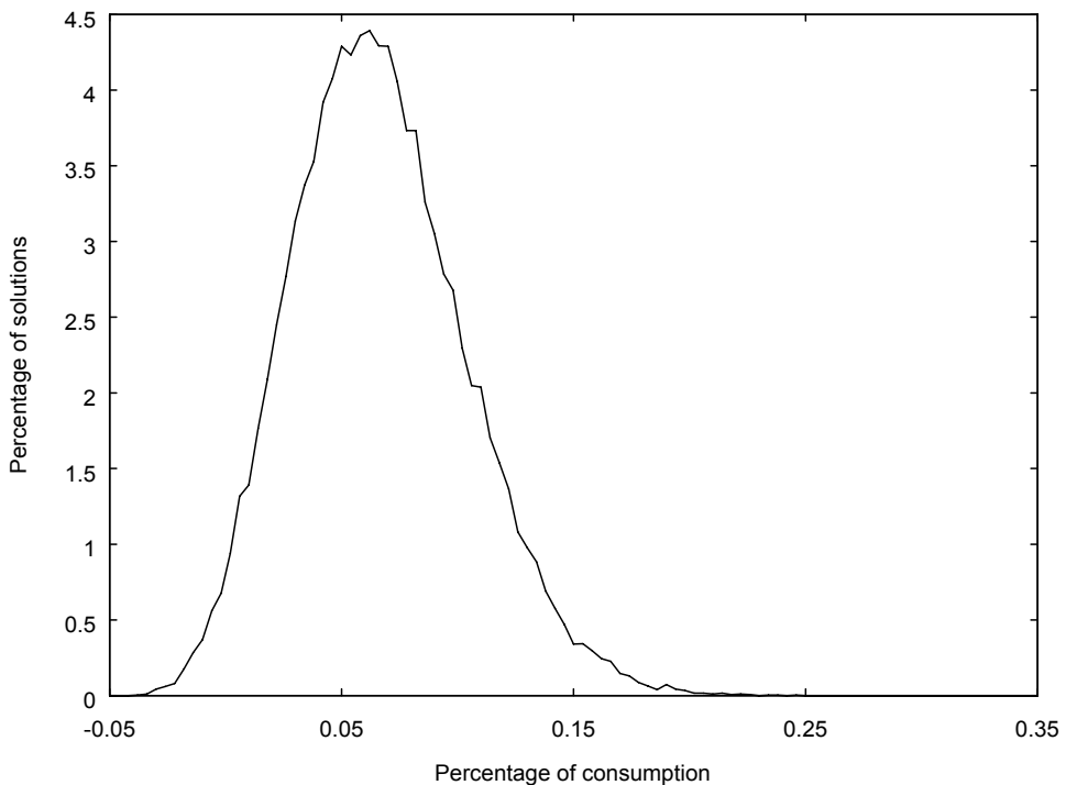
Figure 4: Sample Distribution of the Welfare Results of Armenian-CIS FTA 30,000 simulations.
