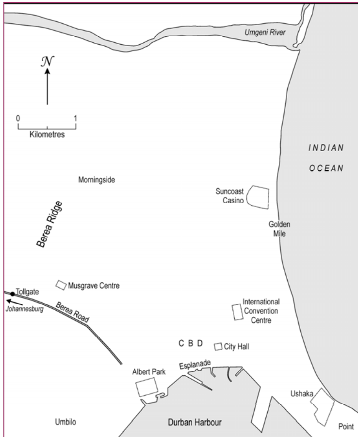
Map 1 Inner Durban
