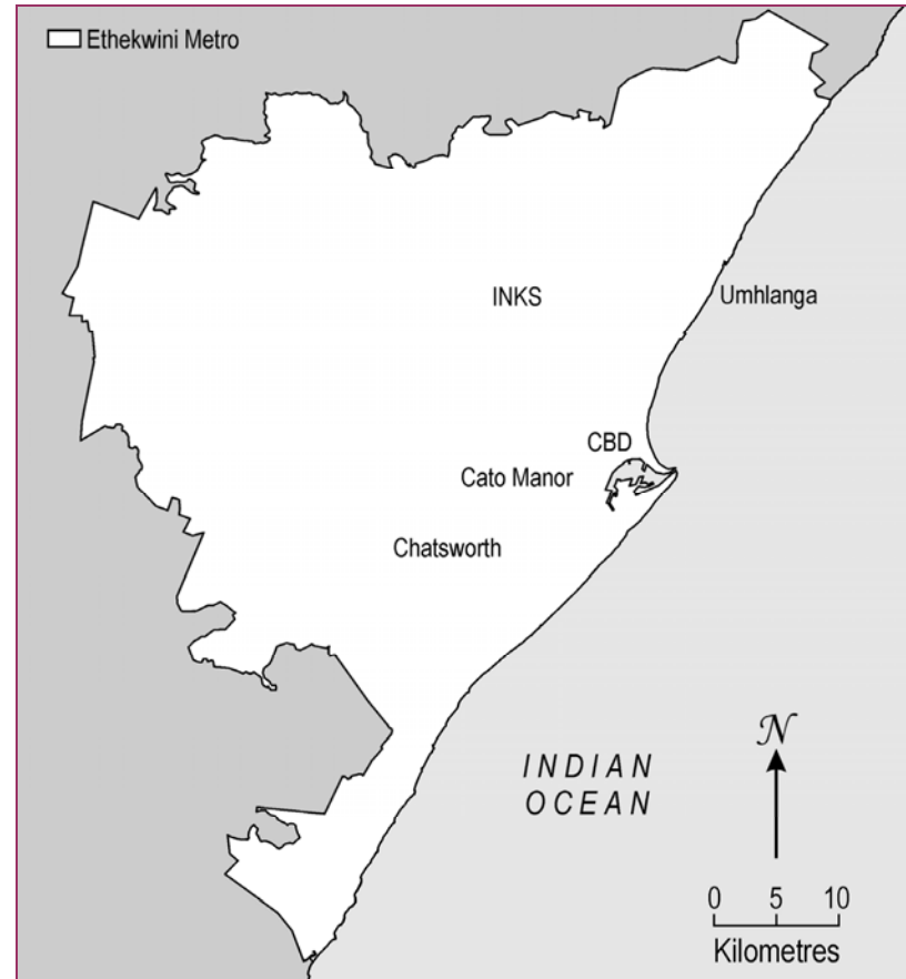
Map 2 Ethekekwini Metro
