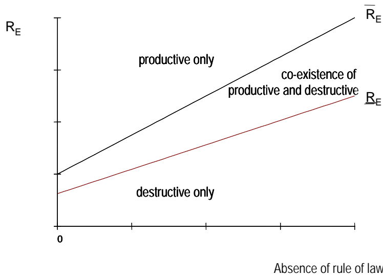
Figure 2: \bar{R}_E and \underline{R}_E as functions of the change in rule of law \lambda
