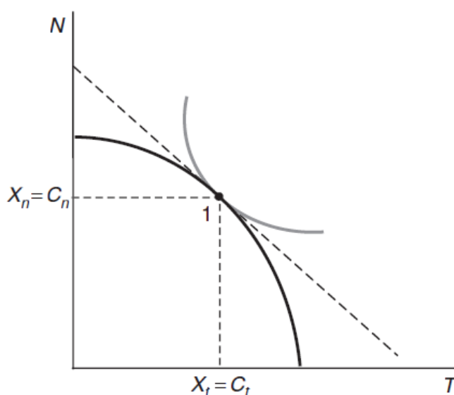
Figure 4: Non-distorted Equilibrium
