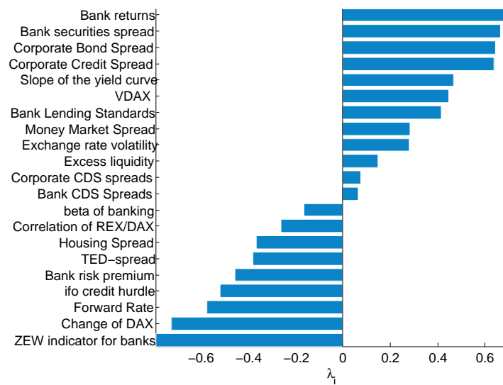
Figure 16: Factor loadings
