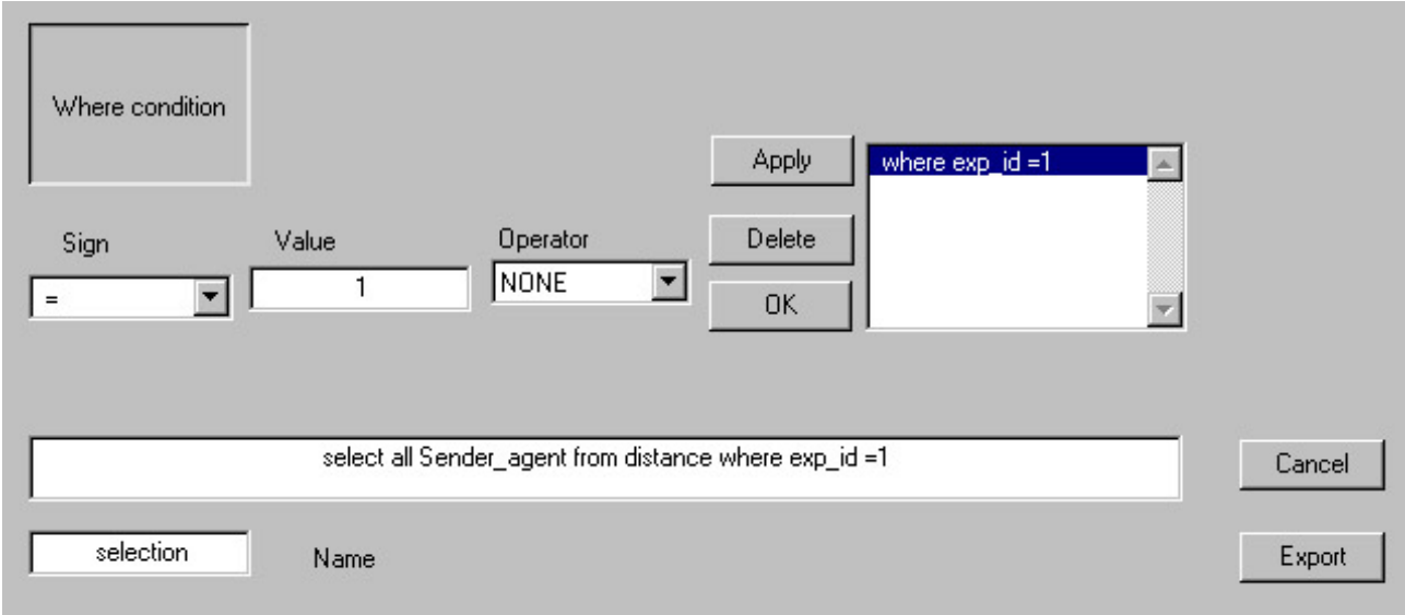
Figure A.9: edit box SQL command
