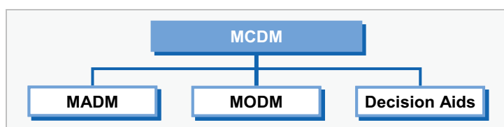
Figure 15: MCDM methodology
