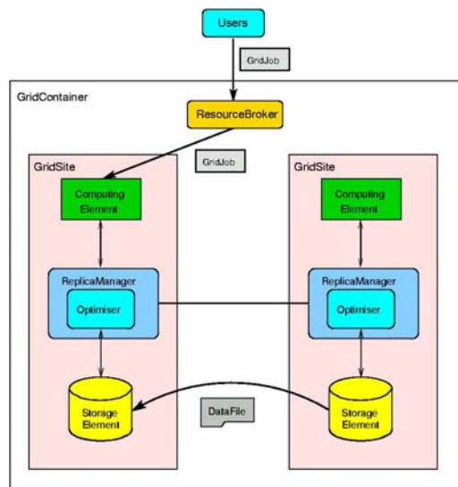
Figure 3.3: OptorSim Architecture.
