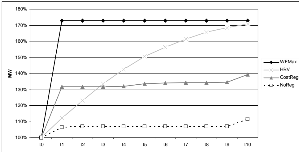
Figure 12: Time path of overall extension in the DRes case for t0-t10
