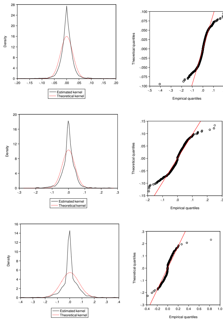
Figure 2: Descriptive graphs
