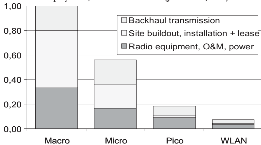
Figure 2 Example of base station cost structure including capex and opex for greenfield deployment, based on data from (Johansson, 2007)
