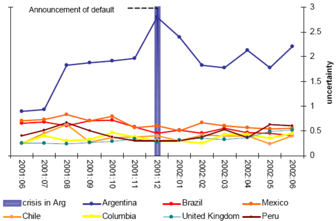
Fig. 2: Evolution of Uncertainty
