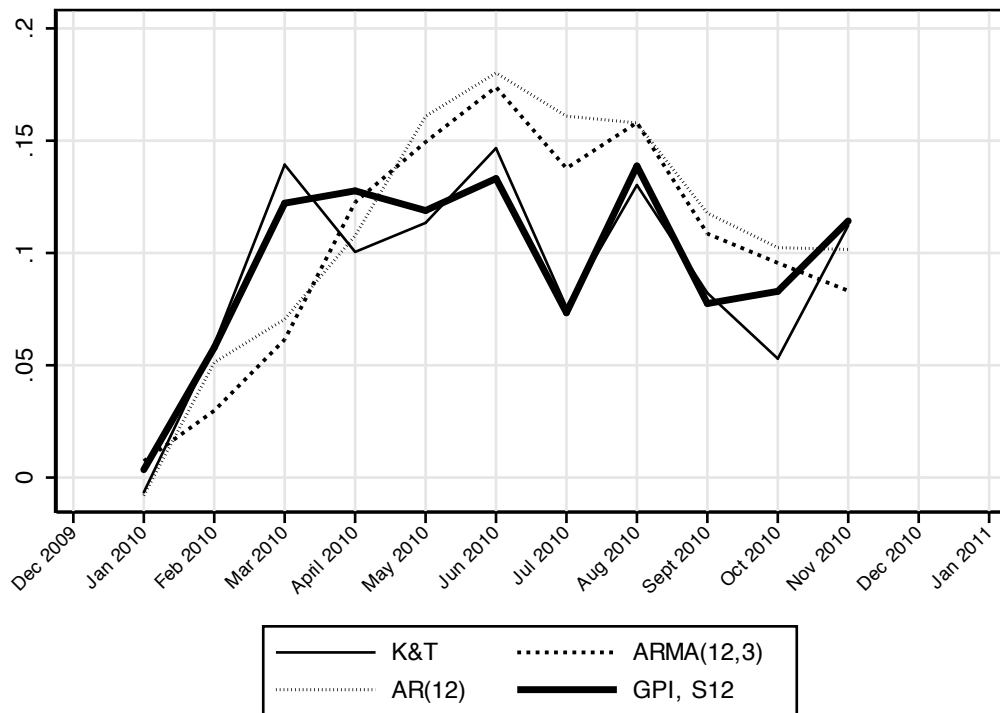
Figure 4: Out of sample performance of the TI model K\&T (which uses TI_k and TI_t ) and AR(12) and ARMA(12, 3) . The TI based forecasting models clearly outperform the AR and ARMA models despite the disadvantage of being estimated on much less data.
