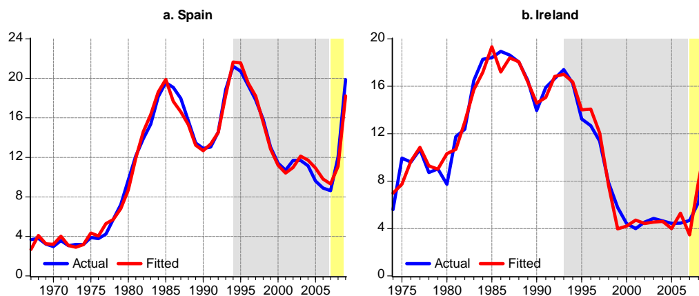
Figure 1. Unemployment rate: Actual and fitted values.
