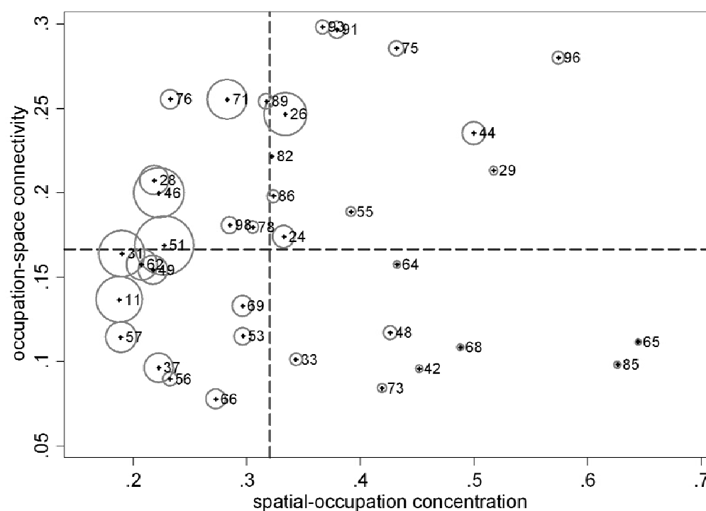
Figure 5 - Spatial occupation concentration and occupation-space connectivity
