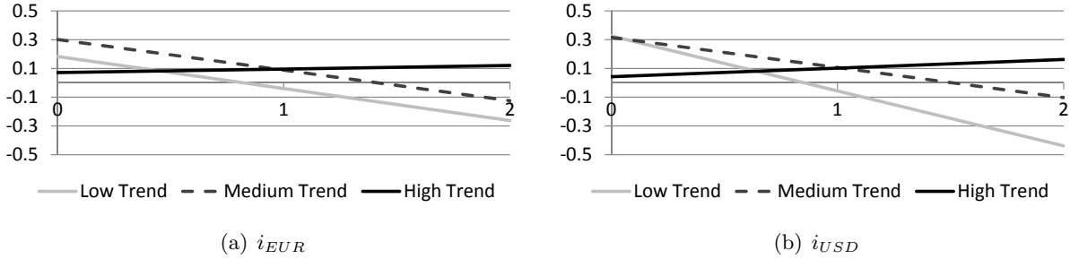
Figure 2: Expected effects of fundamental forecast errors under different momentum phases
