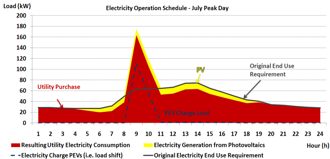
Figure 9: Diurnal Microgrid Analysis for Peak Days in Scenario 1 6
