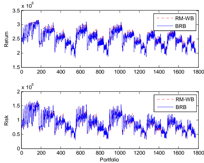
Fig. 7 Comparison between RM-WB and BRB with 9-asset-class portfolios
