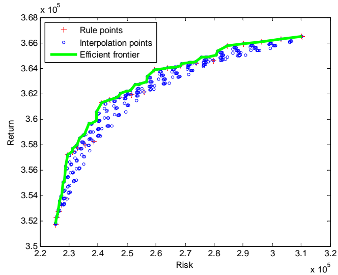
Fig. 6 BRB Efficient frontier for 3-asset-class example
